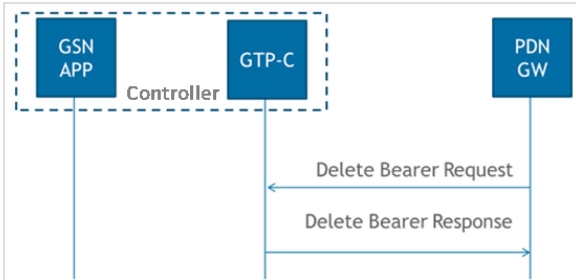
FIGURE 8 Delete bearer
